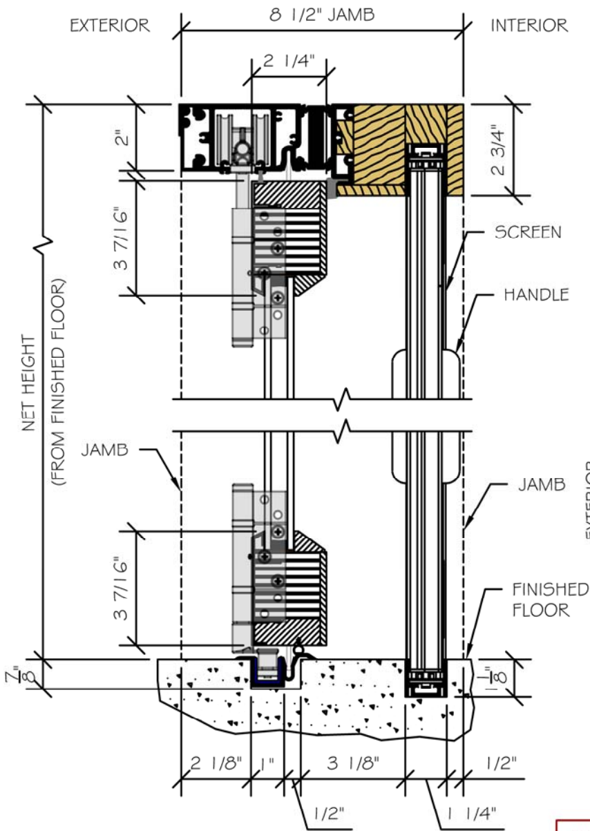
SECTION VIEW
