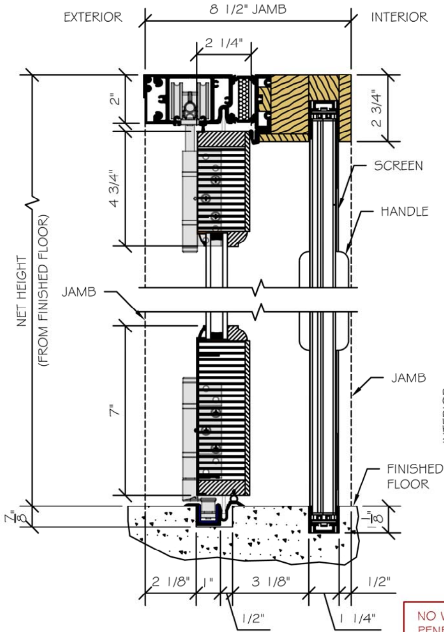
SECTION VIEW
