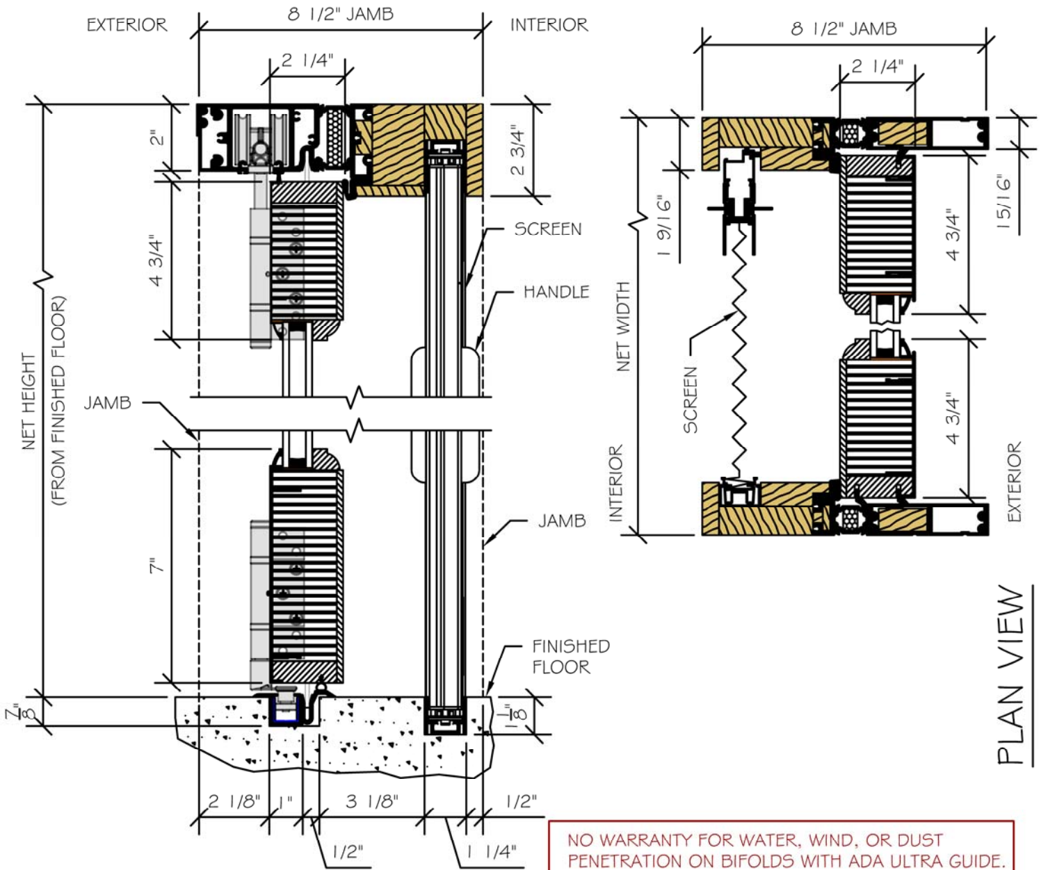
SECTION VIEW
