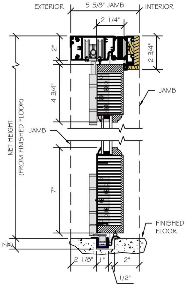
SECTION VIEW
