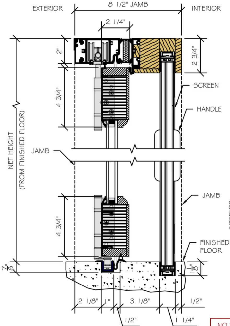
SECTION VIEW
