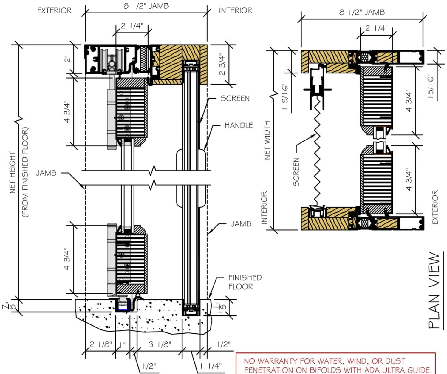
SECTION VIEW
