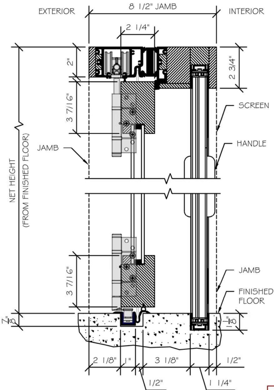
SECTION VIEW
