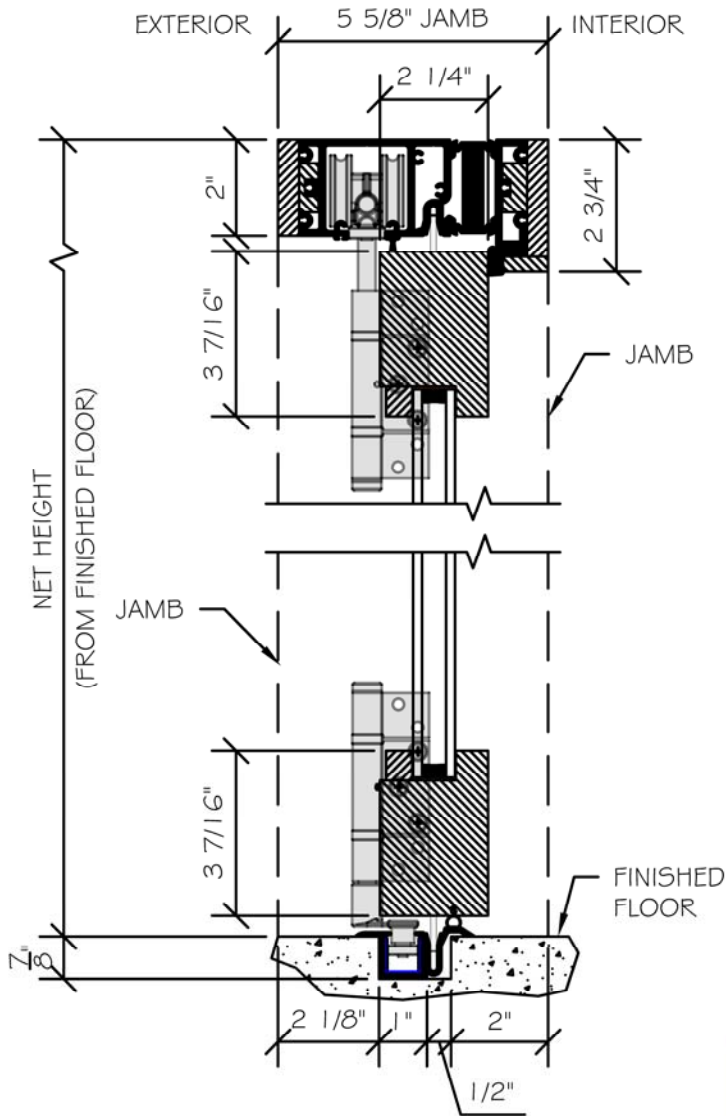
SECTION VIEW
