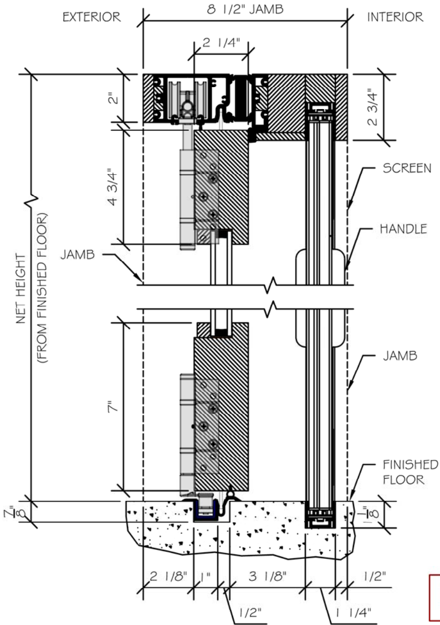
SECTION VIEW
